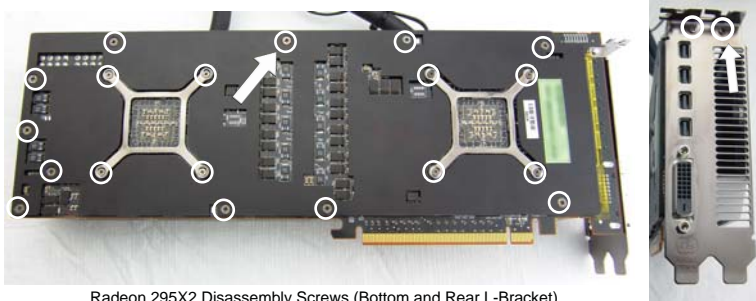
Radeon 295X2 Disassembly Screws (Bottom and Rear L-Bracket)
