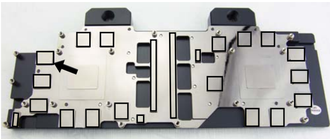
VID-AR295X2 Water Block Thermal Pad Locations
