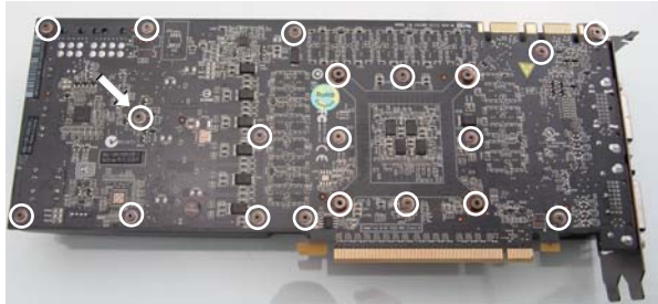
GTX 580 Disassembly Screws (Bottom and Rear L-Bracket)
