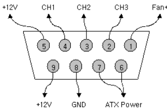
Koolance ERM-2K3U, Exos-2 / V2 / LX / 2.5 / LT V2 Rear DB9 Pin-out
