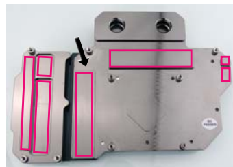
VID-AR697 Thermal Pad Locations
