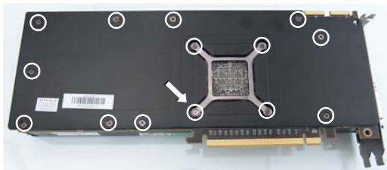
HD 6970 Disassembly Screws
