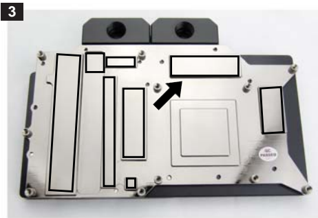
VID-NX1080 Water Block Thermal Pad Locations
