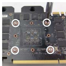
Optional Koolance Back Plate Thermal Pad Locations
