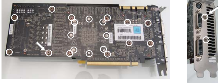
GeForce GTX 285 Disassembly Screws Back Side (Left) and L-Bracket (Right)
