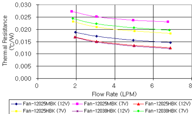
4 Fan AL Radiator (HX-1320) ( \Delta T = \text{Inlet Water} - \text{Ambient} )
