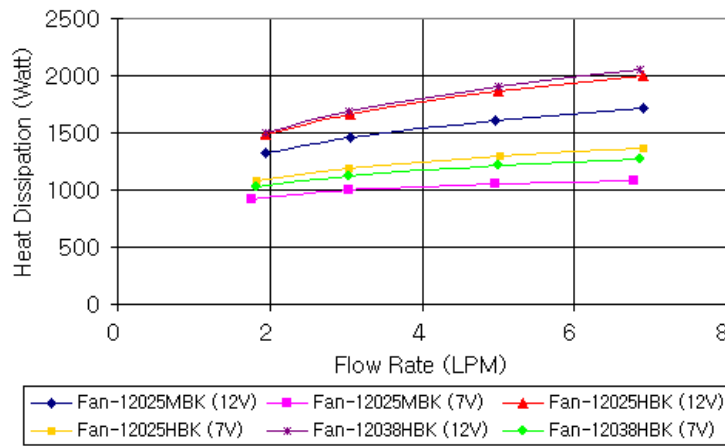
4 Fan AL Radiator (HX-1320) ( \Delta T = \text{Inlet Water} - \text{Ambient} = 25^\circ\text{C} )
