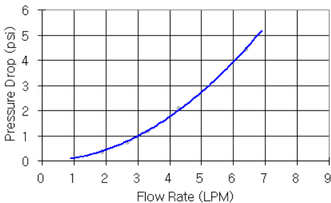
VL2 QDC Nozzle (Straight Male/Female Connection)
