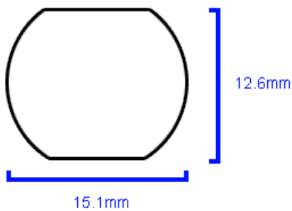
Koolance "VL2" 6mm or 10mm ID Panel Barb Hole Size
