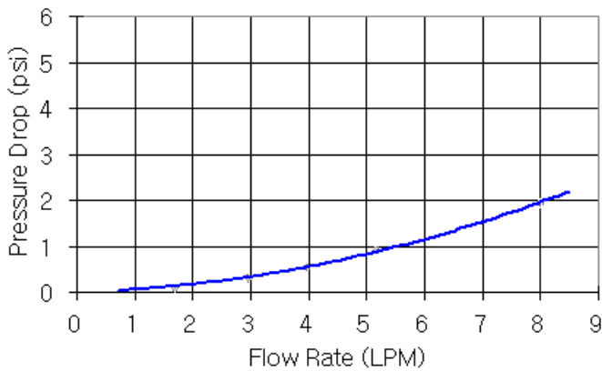
VL3 QDC Nozzle (Straight Male/Female Connection)
