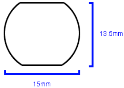
Koolance "VL3" 10mm ID Panel Barb Hole Size
